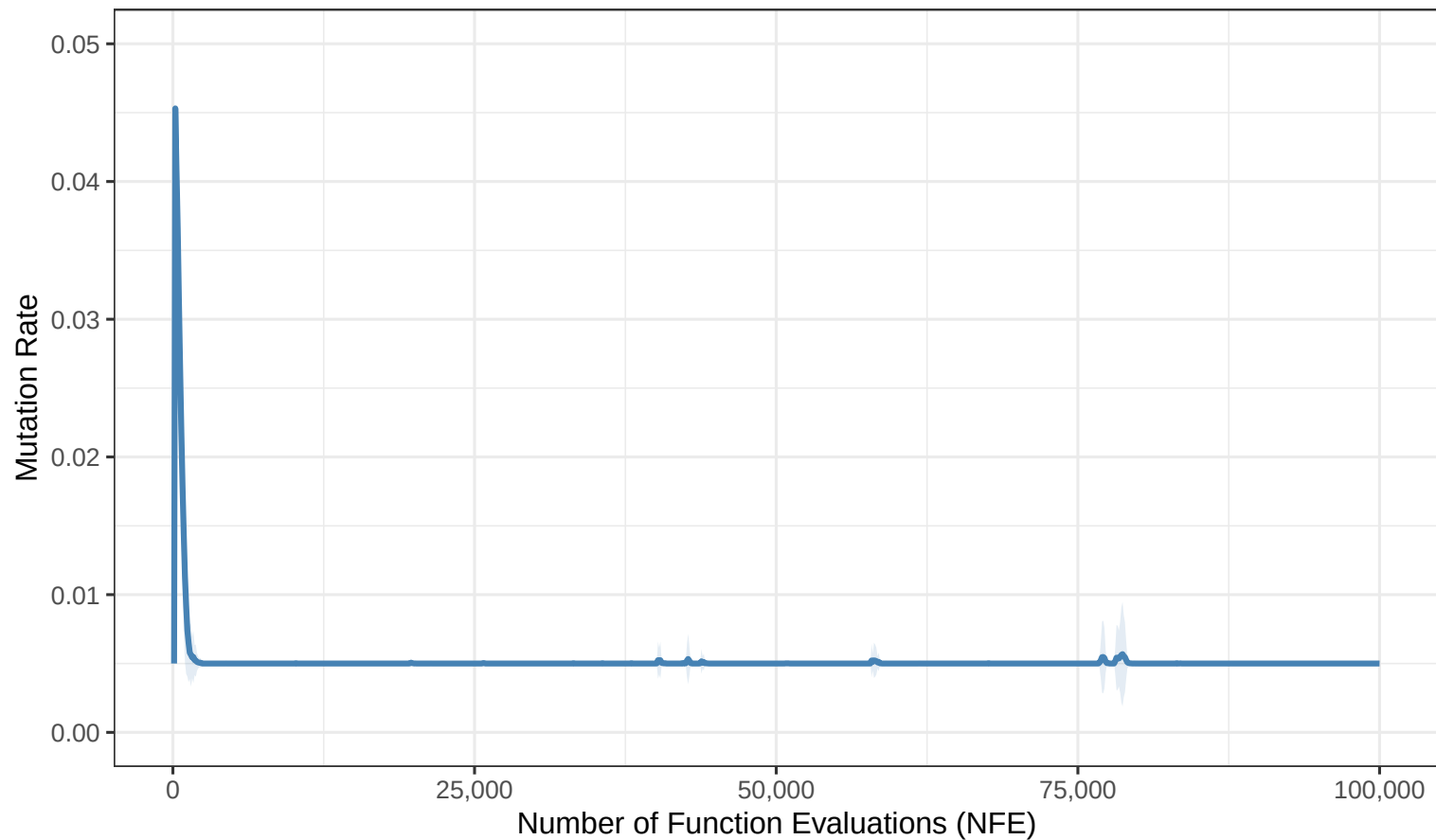
G10 – Adaptive Mutation Rate
