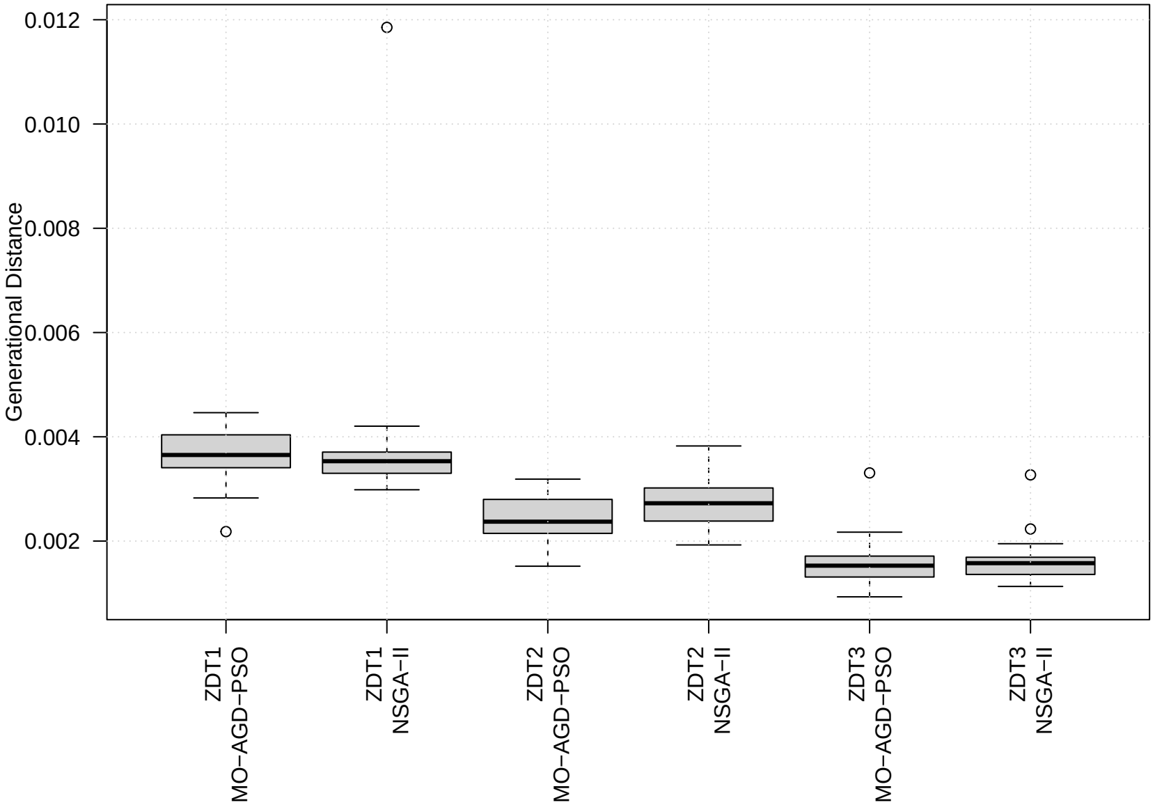
Generational Distance
