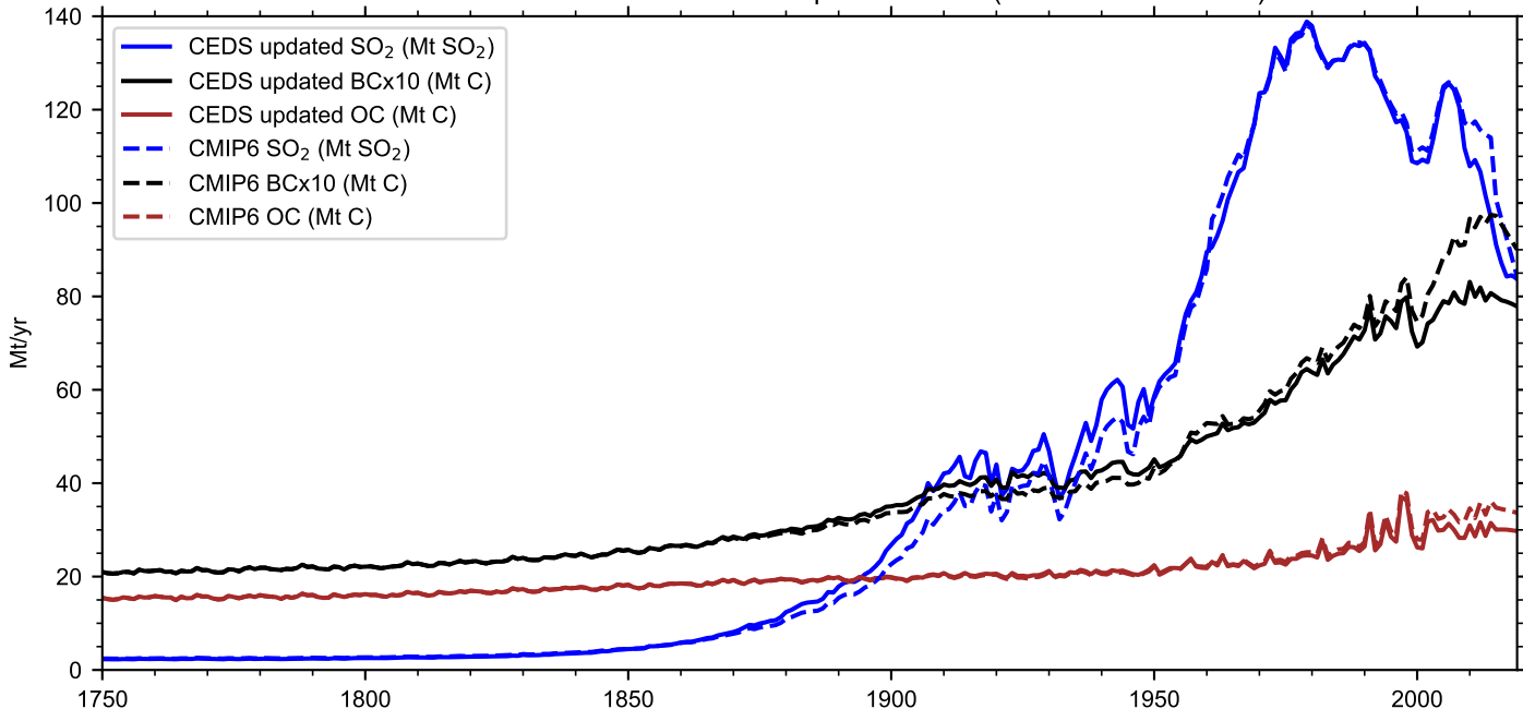
Aerosol emissions from CMIP6 and updated CEDS (O'Rourke et al. 2020)
