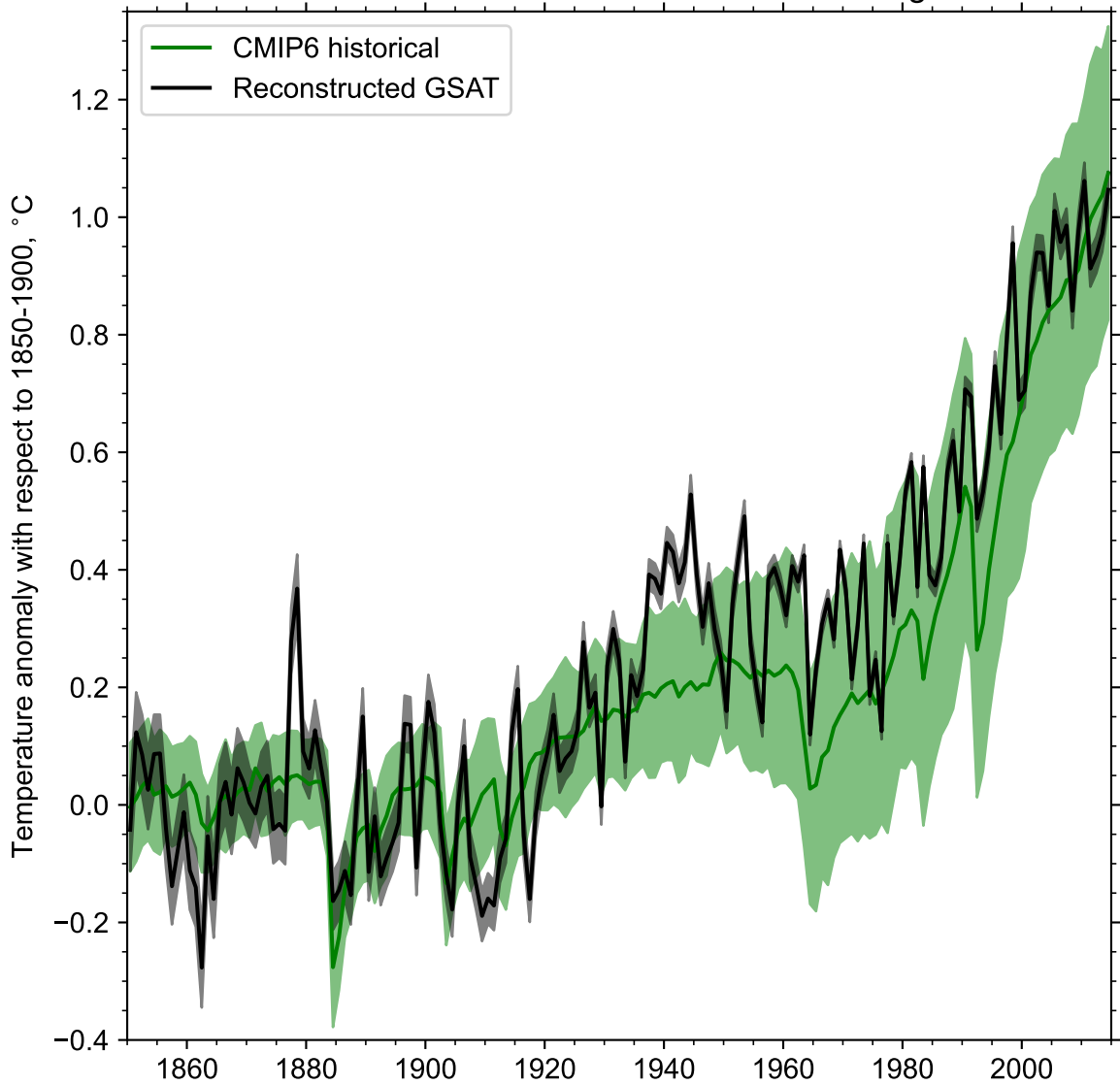
CMIP6 simulated and observed warming
