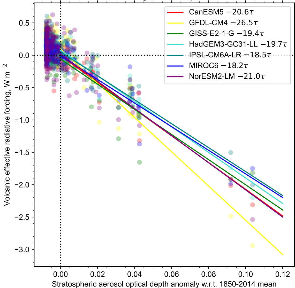
Volcanic forcing in RFMIP piClim-histnat
