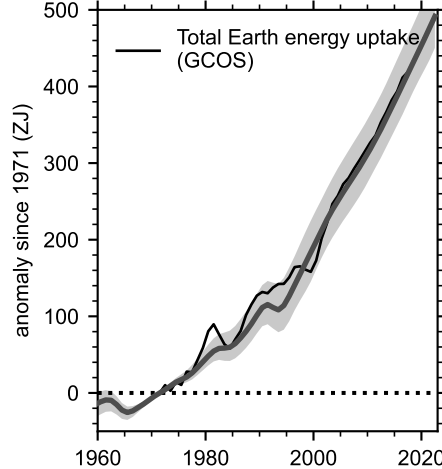
(e) Earth energy uptake
