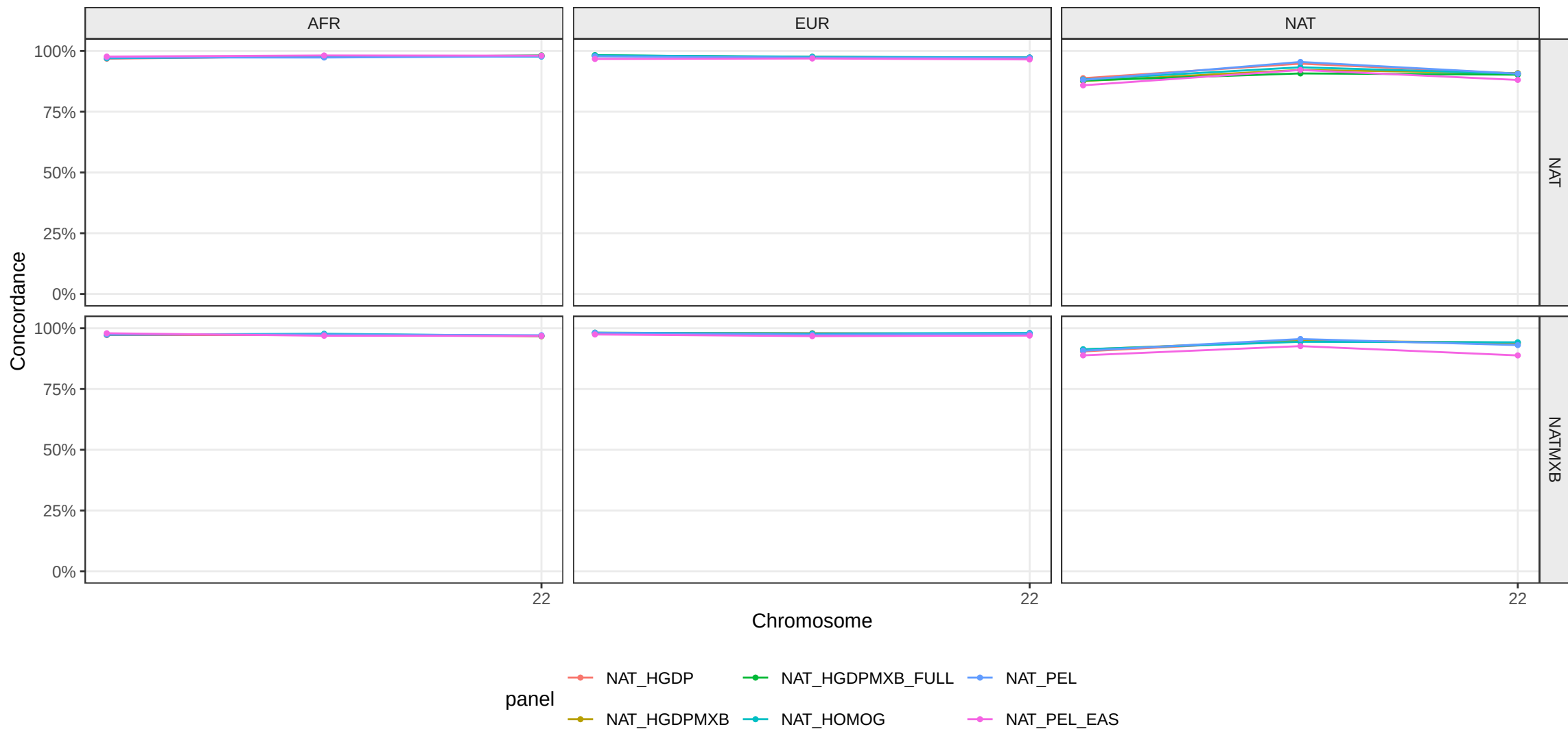
Per-chromosome concordance trajectory by panel
