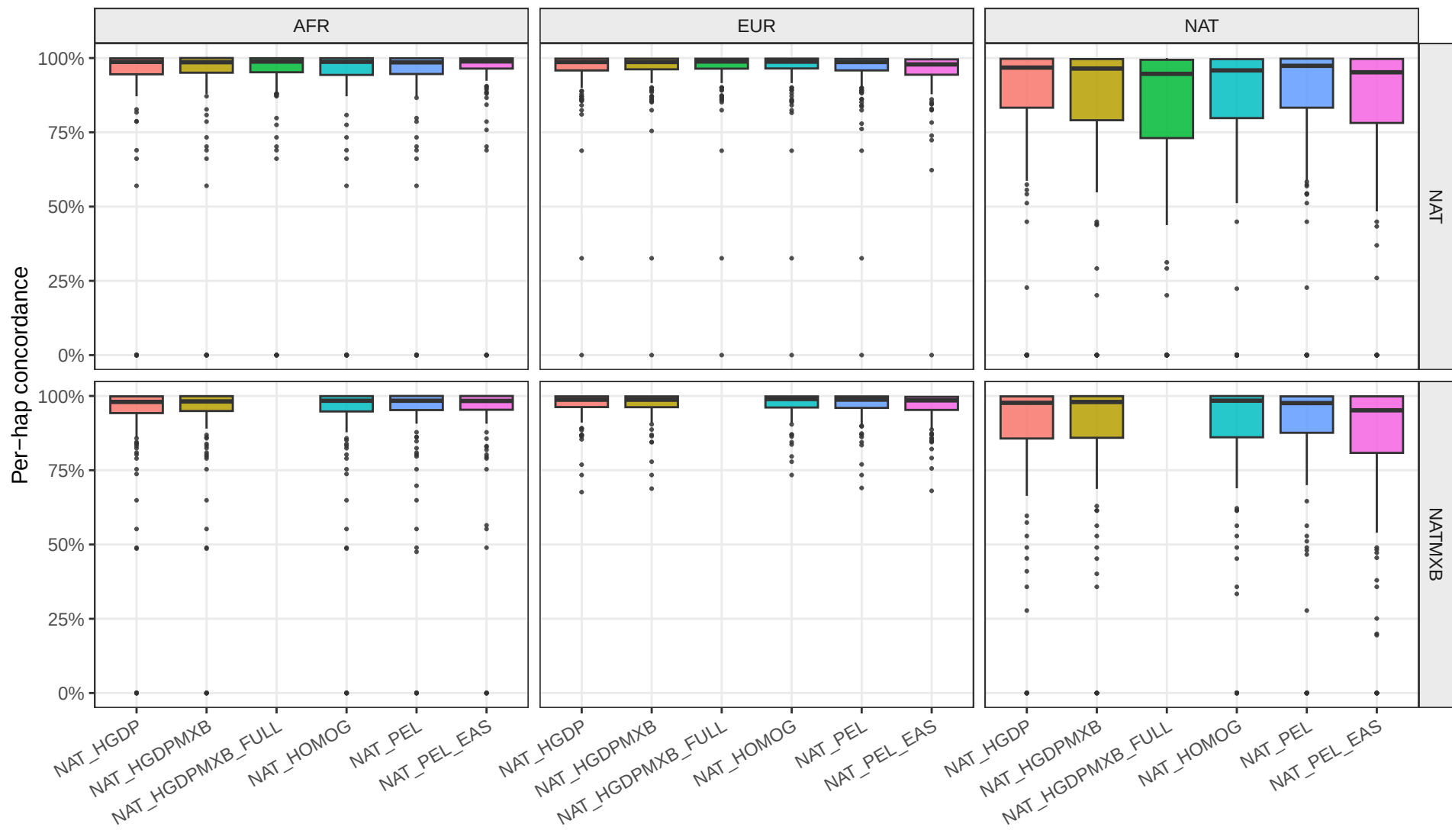
LAI concordance by panel, split by sim track and ancestry
