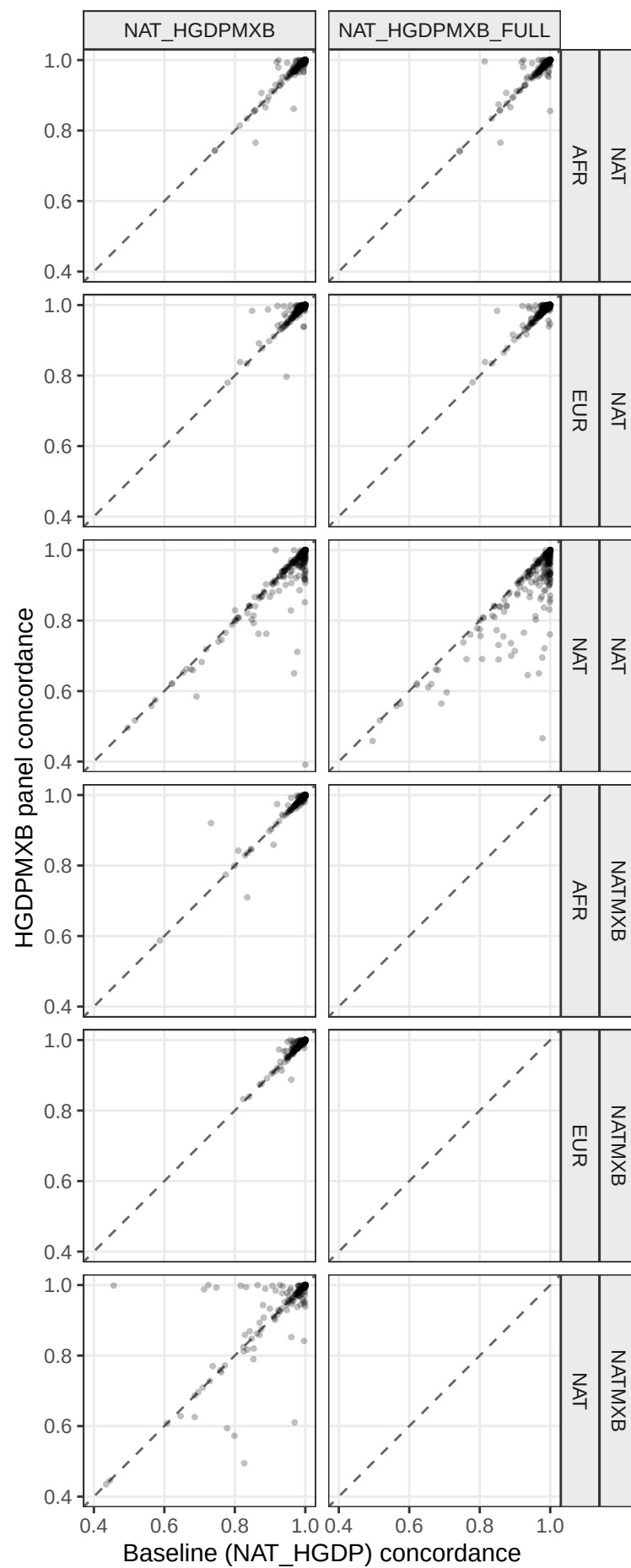
HGDPMXB panels vs. baseline, paired by (chr, hap)
