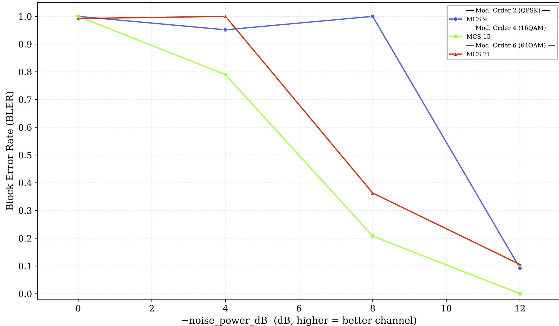
DL BLER for Various MCS Values — BICTR Lunar Channel (RFSim, phy-test mode)
