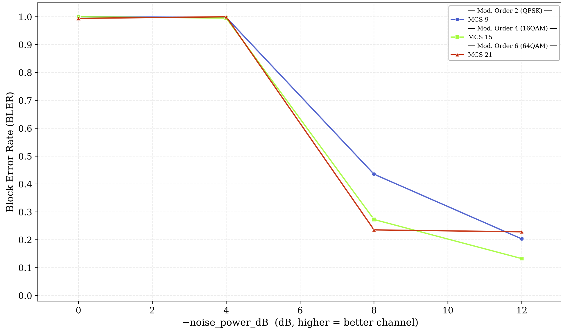
UL BLER for Various MCS Values — BICTR Lunar Channel (RFSim, phy-test mode)
