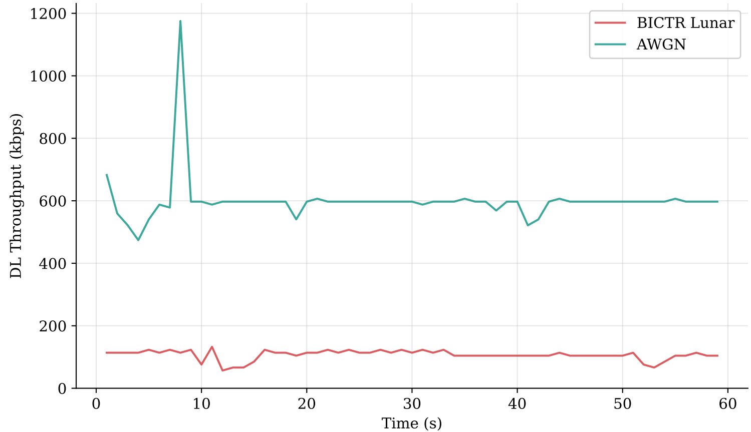
Downlink Throughput Over Time
