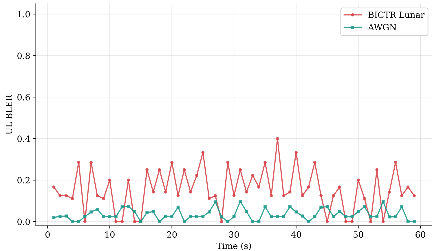
UL Block Error Rate Over Time
