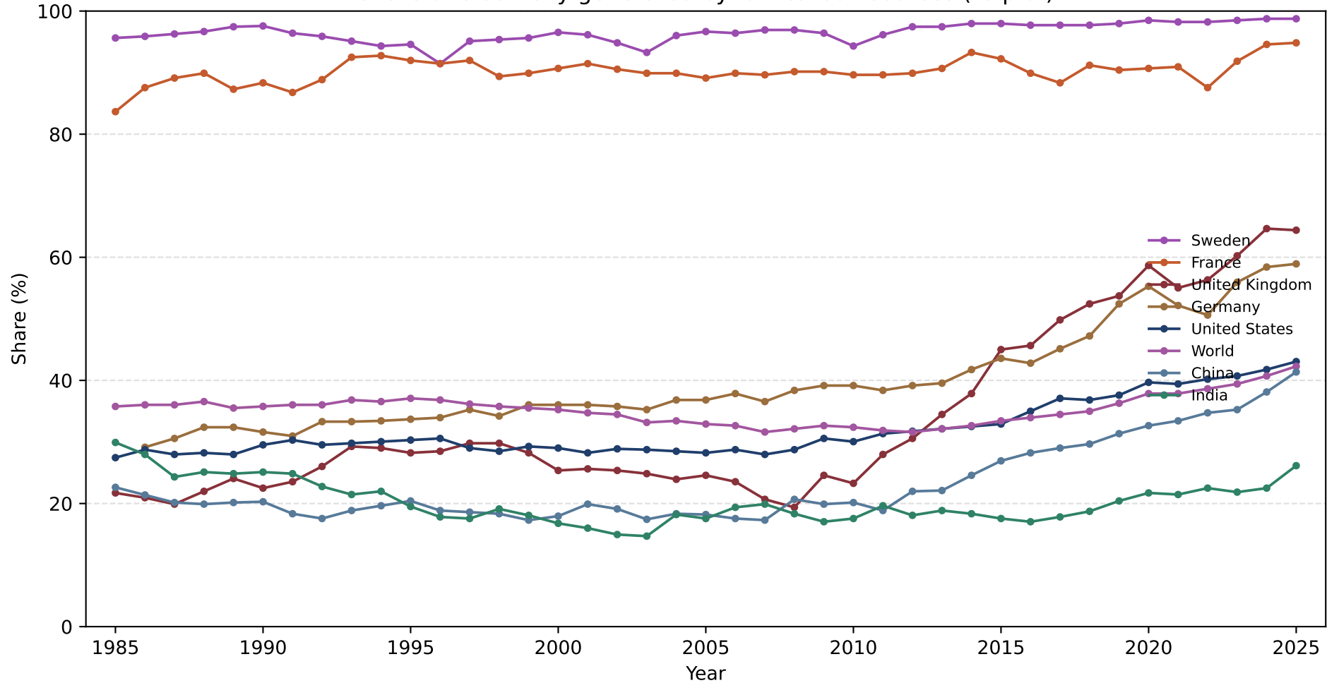
Share of electricity generated by low-carbon sources (re-plot)
