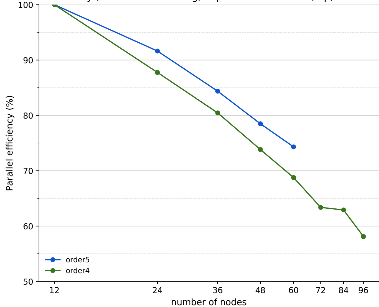
Parallel Efficiency (AltoTiberina Catalog, SuperMUC-NG-Phase1, dp, SeisSol v.1.1.3)
