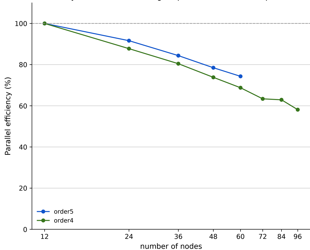
Parallel Efficiency (AltoTiberina Catalog, SuperMUC-NG-Phase1, dp, SeisSol v.1.3.1)
