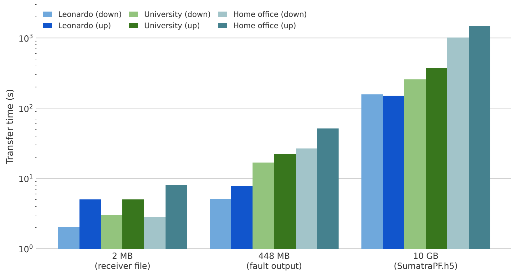
SDL transfer performance (CLI v0.13.55)
