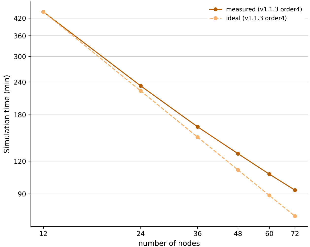
Strong Scaling (AltoTiberina Catalog, SuperMUC-NG-Phase1, dp, SeisSol v1.1.3 order4)
