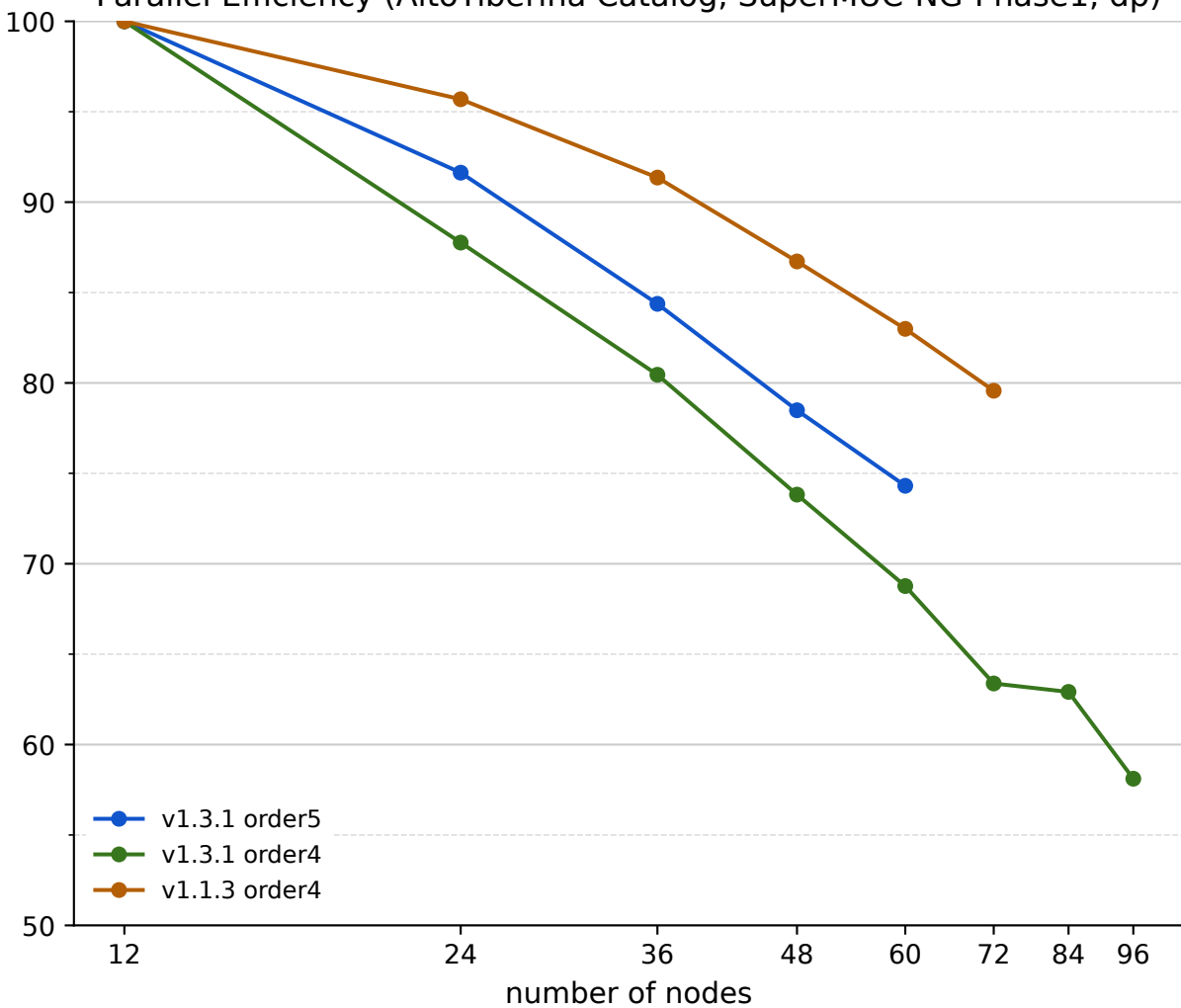
Parallel Efficiency (AltoTiberina Catalog, SuperMUC-NG-Phase1, dp)
