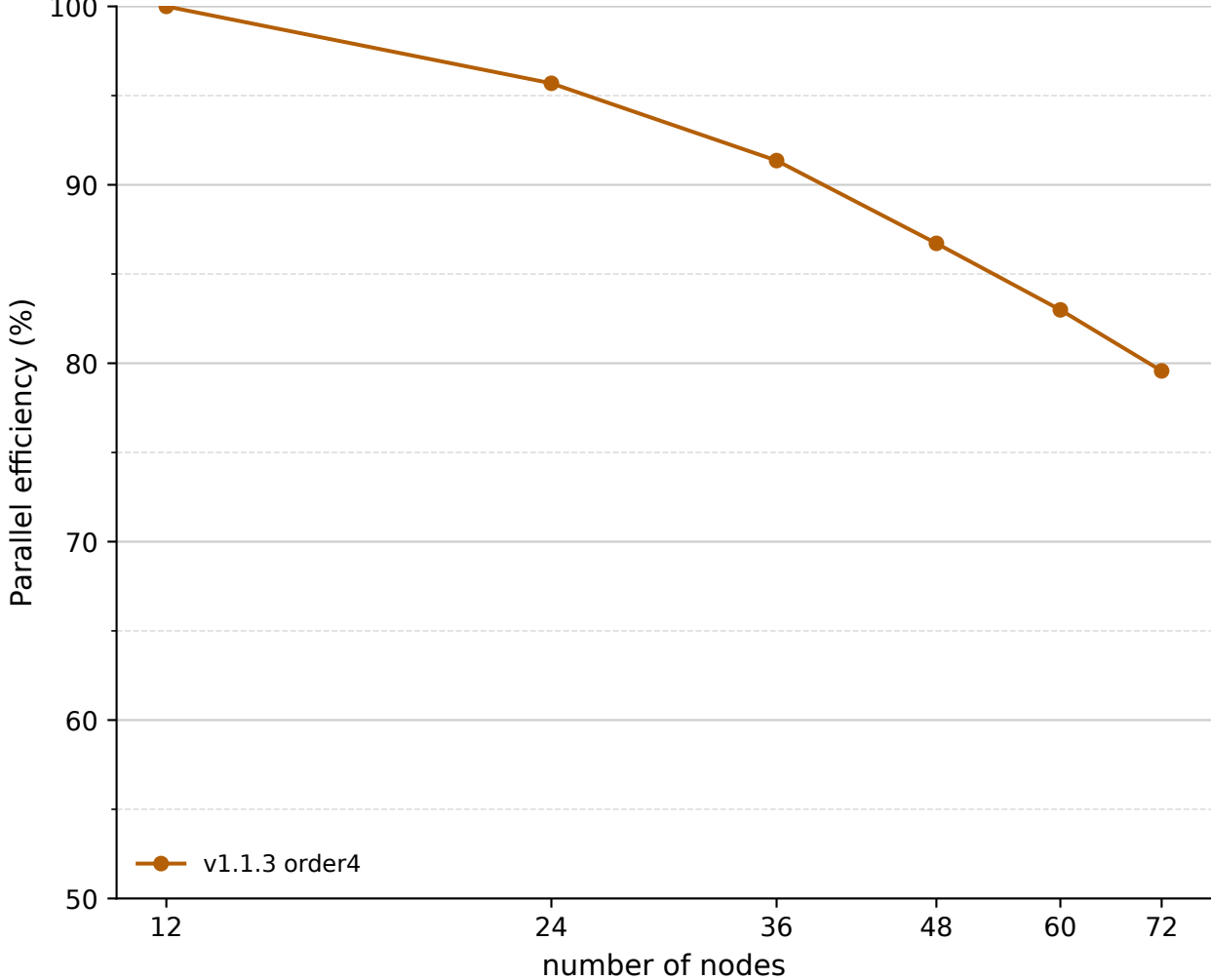
Parallel Efficiency (AltoTiberina Catalog, SuperMUC-NG-Phase1, dp, SeisSol v1.1.3 order4)
