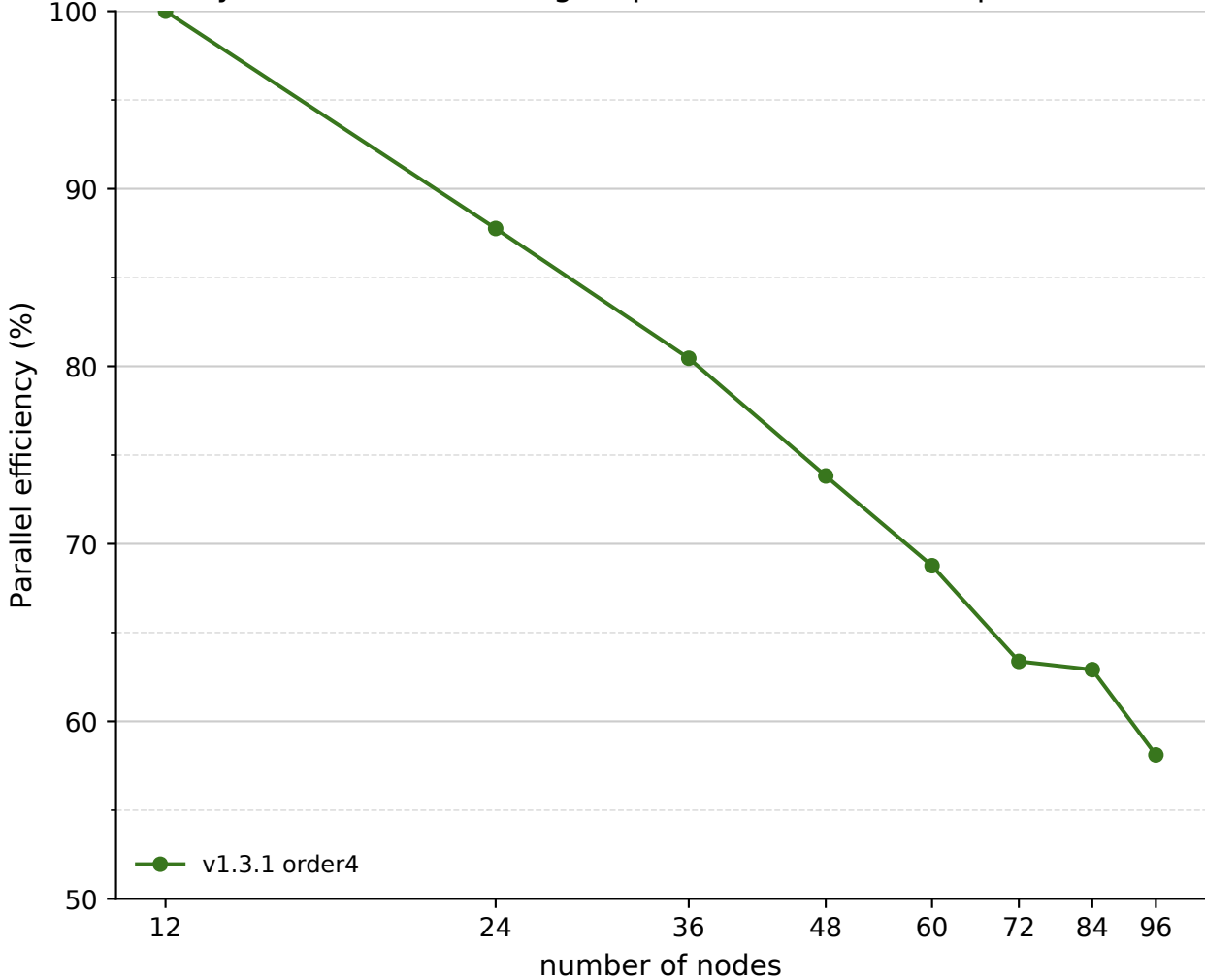
Parallel Efficiency (AltoTiberina Catalog, SuperMUC-NG-Phase1, dp, SeisSol v1.3.1 order4)
