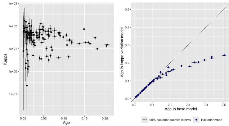
(a) Lineage age (number of expected substitutions per site for the present) vs estimated kappa for carnivores dataset (b) Node age estimates for base model vs per-lineage kappa variation model
