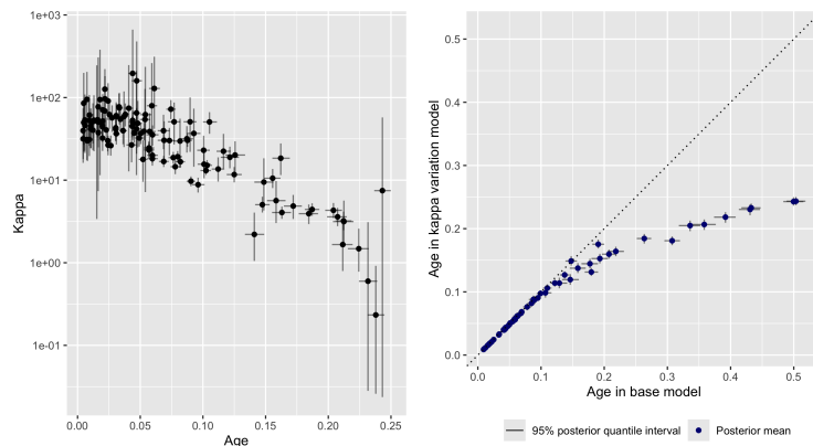
(a) Estimated per-branch kappa (b) Internal node age estimates against the age of each branch. under the two models. Each point is the posterior mean point is one internal node, with its of the kappa parameter for one age under the base (single-kappa) branch, shown on a logarithmic model on the horizontal axis and scale; the vertical bars show its age under the per-branch kappa 95% credible interval and the horizontal bars show the 95% credible interval of the age. Age is the height of the branch's midpoint interval, and the dotted line is above the present, measured in expected substitutions per site (the tree is estimated in units of substitutions and is not calibrated to time).
