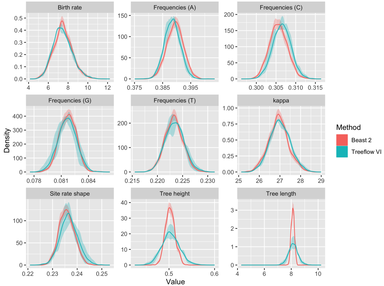
Fig. 2: Posterior marginal parameter estimates for the carnivores base model (a single transition/transversion ratio, kappa, shared across the whole tree), comparing TreeFlow variational inference (Treeflow VI, teal) with BEAST 2 MCMC (Beast 2, red). The solid curves show the estimated marginal posteriors and the shaded bands represent the Monte Carlo error of each estimate. For BEAST 2 the band is obtained by bootstrapping the MCMC samples; for TreeFlow VI it is estimated from the variability between four independent variational runs, with the curve showing the posterior pooled across those runs.
