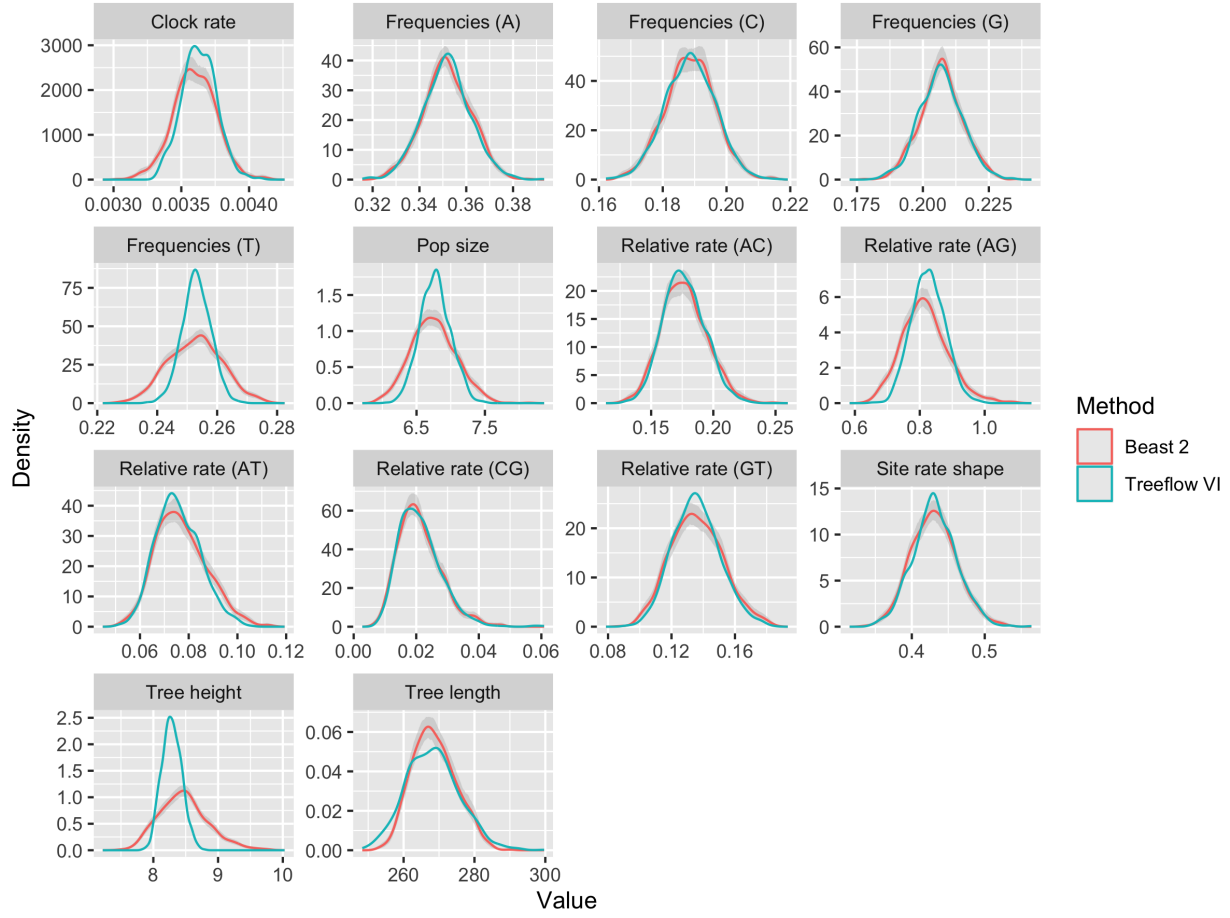
(a) Marginal posterior distributions for the model parameters, comparing TreeFlow variational inference (Treeflow VI, teal) with BEAST 2 MCMC (Beast 2, red). As in Figure 2, the grey band around each BEAST 2 density shows the Monte Carlo sampling error of the MCMC estimate, obtained by bootstrapping the MCMC samples.
