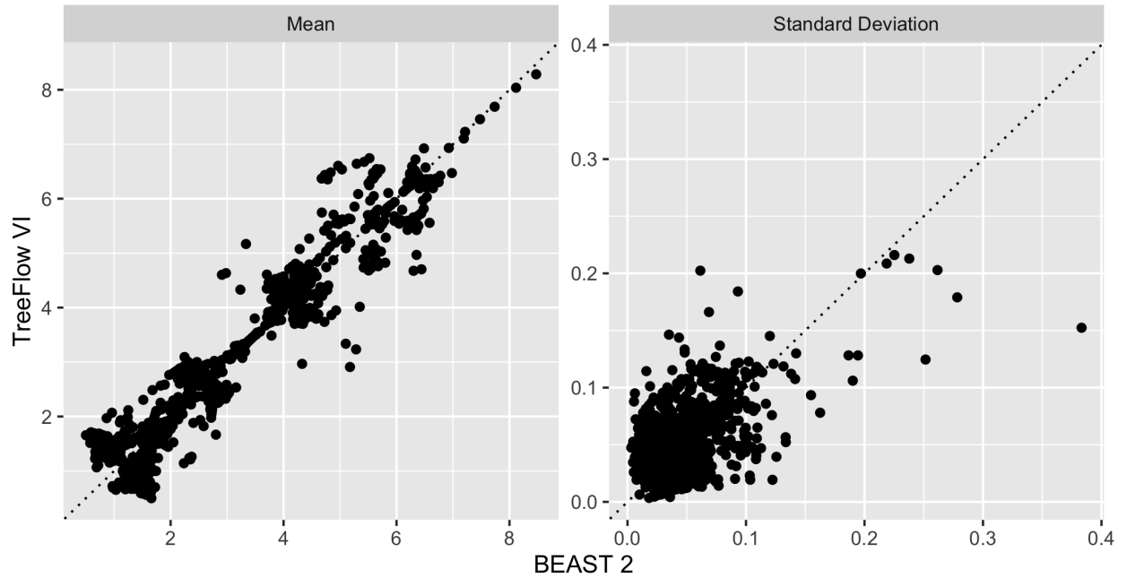
(b) Per-node summaries of the internal node height posteriors, plotting the TreeFlow VI estimate against the BEAST 2 estimate for each node. The left panel compares the posterior means and the right panel the posterior standard deviations; the dotted line in each panel is the identity. Standard-deviation points falling below the identity indicate node heights whose posterior uncertainty is underestimated by the mean-field variational approximation relative to BEAST 2.
