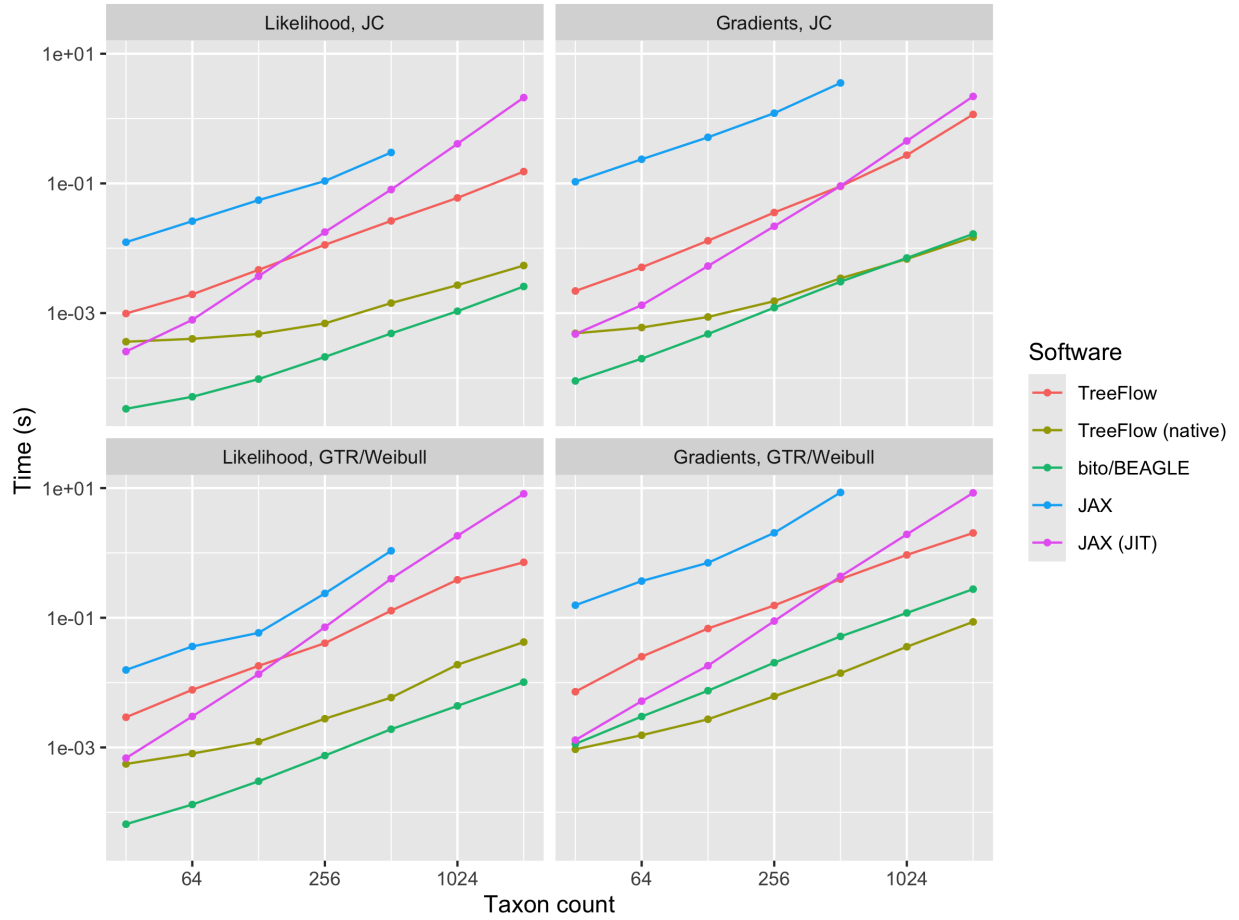
Figure 5: Times from the phylogenetic likelihood benchmark, on log-log axes. Each point is the time for a single evaluation of the computation on an alignment of 1000 sites, averaged over 10 simulated datasets. Each panel corresponds to one of the four benchmarked computations (likelihood and gradient evaluation, under the simple JC model and the more complex GTR/Weibull model), with the five implementations plotted as separate series: TreeFlow’s portable TensorArray traversal (TreeFlow) and its native C++ operation (TreeFlow (native)), bito/BEAGLE, and the eager (JAX) and JIT-compiled (JAX (JIT)) JAX implementations. Eager JAX is only run up to 512 taxa as its runtime becomes prohibitive on larger trees.
