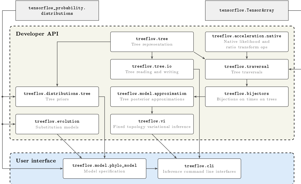
Figure 1: Diagram showing the architecture of the TreeFlow package. Nodes represent Python modules and the arrows between them denote major dependencies. The dashed rectangles separate the components based on their primary interfaces. Nodes outside the two interface groups denote major external dependencies.
