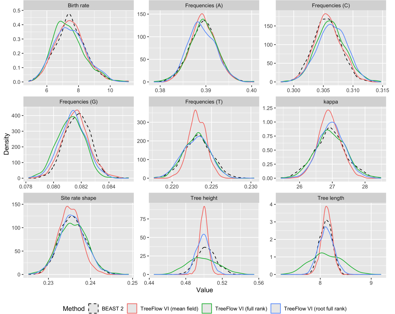
Figure S3: Posterior marginals for the carnivores dataset under each of TreeFlow’s three variational approximation families (solid lines), against the BEAST 2 reference posterior (dashed). One variational run per family.
