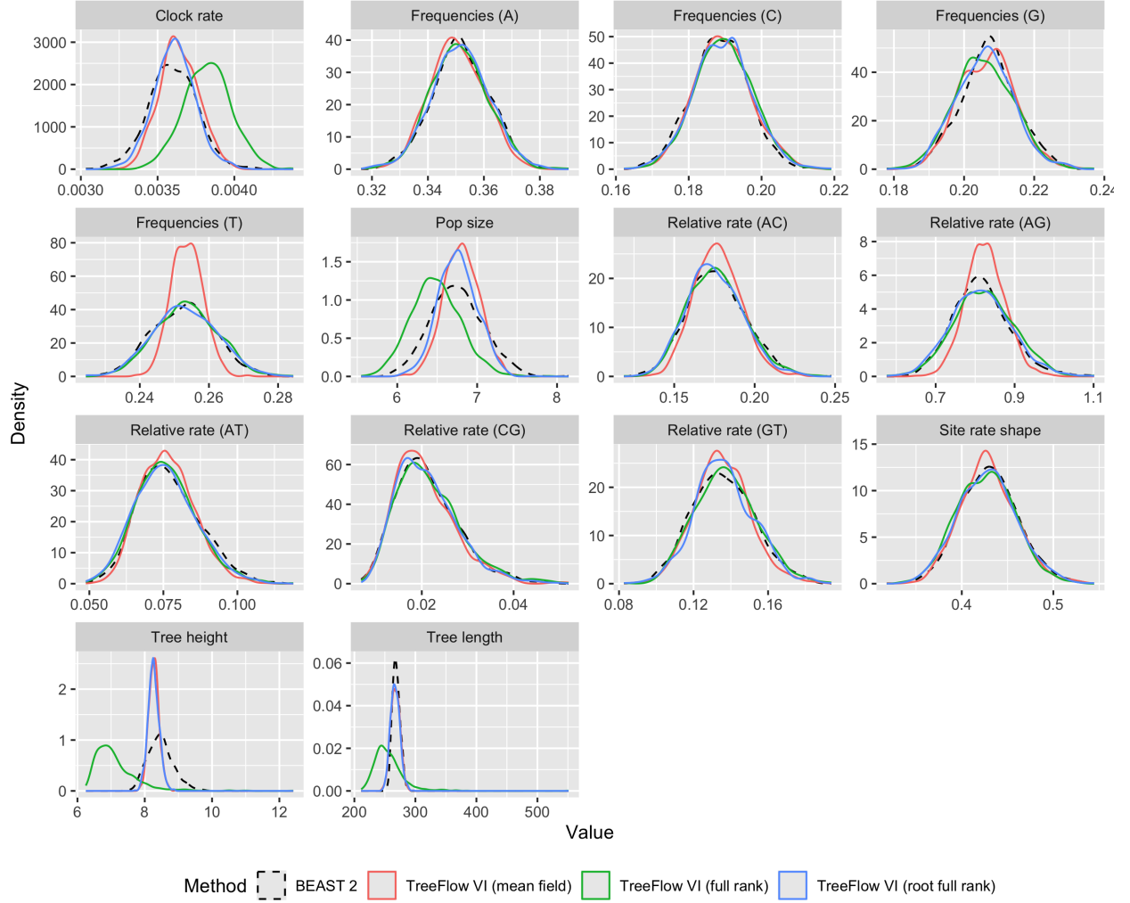
Figure S4: Posterior marginals for the influenza (H3N2) dataset under each of TreeFlow's three variational approximation families (solid lines), against the BEAST 2 reference posterior (dashed). One variational run per family.
