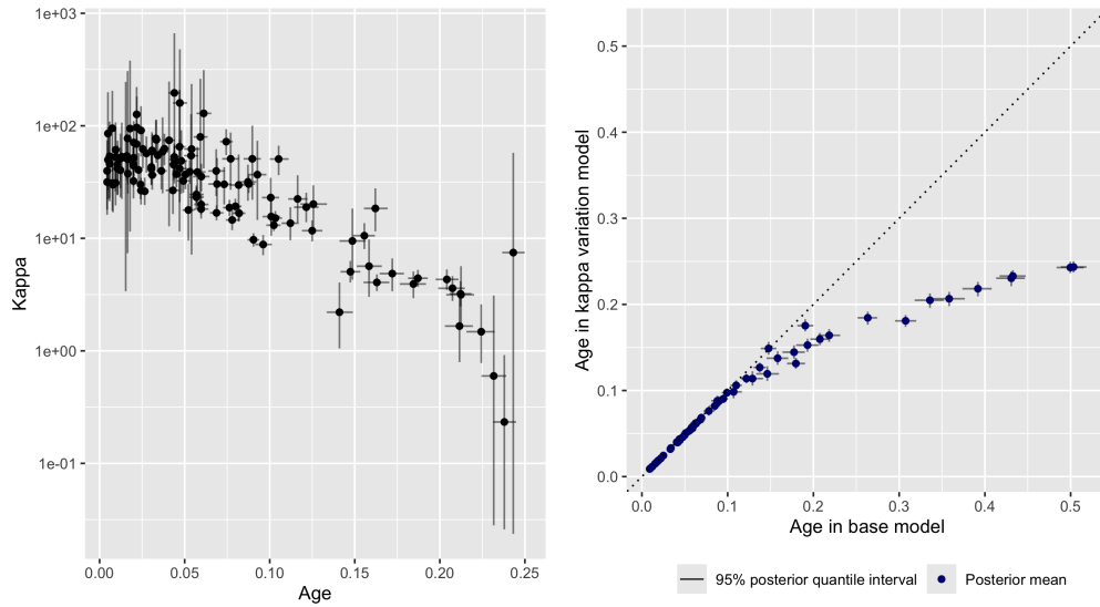
(a) Estimated per-branch kappa against the (b) Internal node age estimates under the two age of each branch. Each point is the posterior models. Each point is one internal node, with mean of the kappa parameter for one branch, its age under the base (single-kappa) model on shown on a logarithmic scale; the vertical bars the horizontal axis and its age under the per- show its 95% credible interval and the horizon- branch kappa variation model on the vertical tal bars show the 95% credible interval of the axis; points are posterior means, bars show the age. Age is the height of the branch's midpoint 95% posterior quantile interval, and the dot- above the present, measured in expected sub- ted line is the identity. Points falling below the stitutions per site (the tree is estimated in units identity for older nodes show that the kappa of substitutions and is not calibrated to time); it is therefore not the branch length. variation model infers younger ages for deeper nodes.
