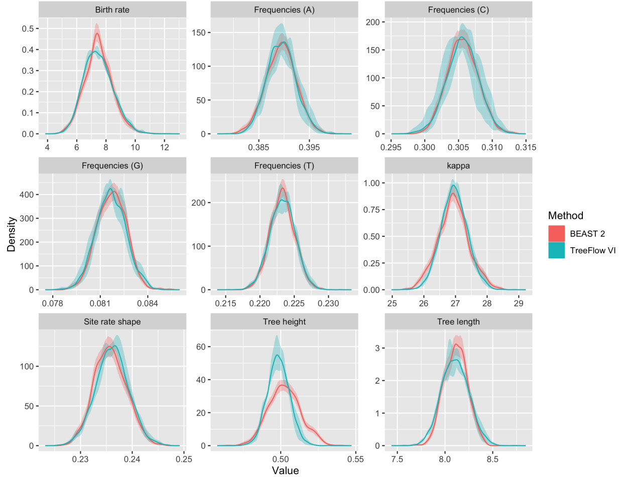
Fig. 2: Carnivores base model posterior Posterior marginal parameter estimates for the carnivores base model (a single transition/transversion ratio, kappa, shared across the whole tree), comparing TreeFlow variational inference (Treeflow VI, teal) with BEAST 2 MCMC (Beast 2, red). The solid curves show the estimated marginal posteriors and the shaded bands represent the Monte Carlo error of each estimate. For BEAST 2 the band is obtained by bootstrapping the MCMC samples; for TreeFlow VI it is estimated from the variability between four independent variational runs, with the curve showing the posterior pooled across those runs. The variational runs use the root full rank approximation; the corresponding comparison of all three approximation families is given in Supplementary Appendix Figure S3.
