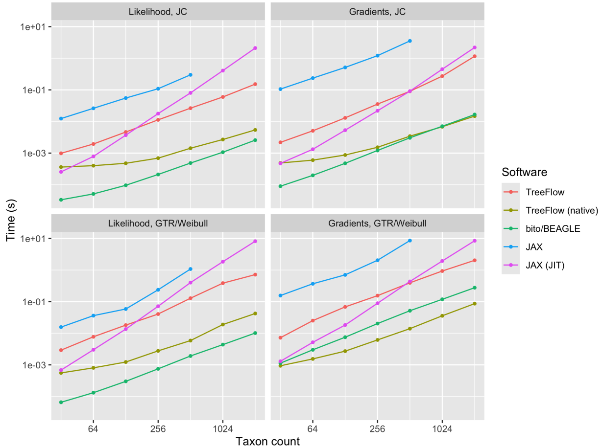
Fig. 5: Times from the phylogenetic likelihood benchmark (100 evaluations), on log-log axes. Each point is the time for a single evaluation of the computation on an alignment of 1000 sites, averaged over 10 simulated datasets. Each panel corresponds to one of the four benchmarked computations (likelihood and gradient evaluation, under the simple JC model and the more complex GTR/Weibull model), with the five implementations plotted as separate series: TreeFlow's portable TensorArray traversal (TreeFlow) and its native C++ operation (TreeFlow (native)), bito/BEAGLE, and the eager (JAX) and JIT-compiled (JAX (JIT)) JAX implementations. This layout makes the differences in scaling (the slope of each series) between the implementations directly comparable within each computation. Eager JAX is only run up to 512 taxa as its runtime becomes prohibitive on larger trees.
