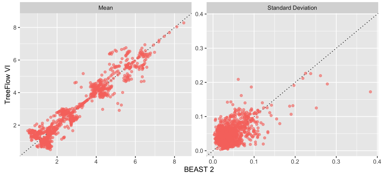
(b) Node Per-node summaries of the internal node height posteriors, plotting the TreeFlow VI estimate against the BEAST 2 estimate for each node. The left panel compares the posterior distribution statistics means and the right panel the posterior standard deviations; the dotted line in each panel is the identity. Points above the identity in
