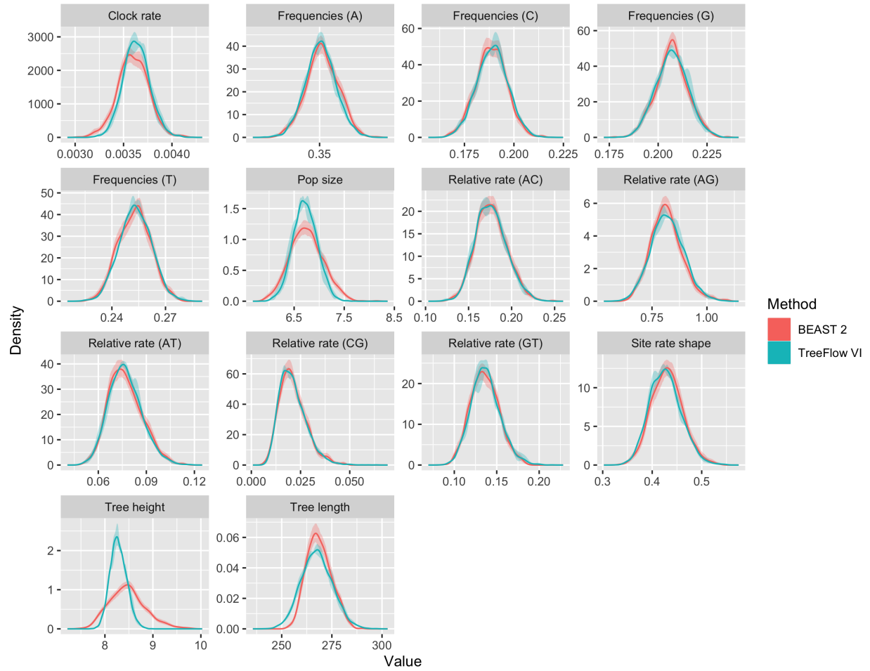
(a) Parameter-marginal Marginal posterior distributions for the model parameters, comparing TreeFlow variational inference (Treeflow VI, teal) with BEAST 2 MCMC (Beast 2, red). As in Figure 2, the shaded band around each curve represents the Monte Carlo error of that estimate: for BEAST 2 it is obtained by bootstrapping the MCMC samples, and for TreeFlow VI from the variability between four independent variational runs, with the curve showing the posterior pooled across those runs. The variational runs use the root full rank approximation; Supplementary Appendix Figure S4 gives the corresponding comparison of all three approximation families.
