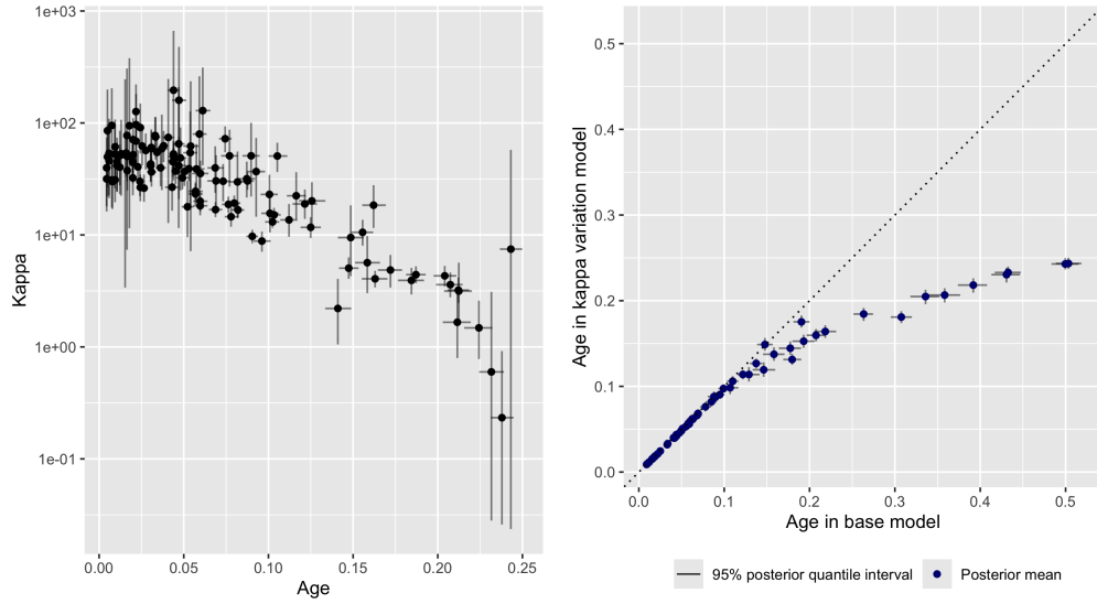
(a) Lineage—Estimated per-branch kappa against the age (number of each branch. Each point is the posterior mean of the kappa parameter for one branch, shown on a logarithmic scale; the vertical bars show its 95% credible interval and the horizontal bars show the 95% credible interval of the age. Age is the height of the branch's midpoint above the present, measured in expected substitutions per site before (the present) vs tree is estimated kappa for carnivores dataset in units of substitutions and is not calibrated to time); for deeper nodes, it is therefore not the branch length. (b) Node—Internal node age estimates for under the two models. Each point is one internal node, with its age under the base (single-kappa) model vs per-lineage on the horizontal axis and its age under the per-branch kappa variation model on the vertical axis; points are posterior means, bars show the 95% posterior quantile interval, and the dotted line is the identity. Points falling below the identity for older nodes show that the kappa variation model infers younger ages for deeper nodes.
