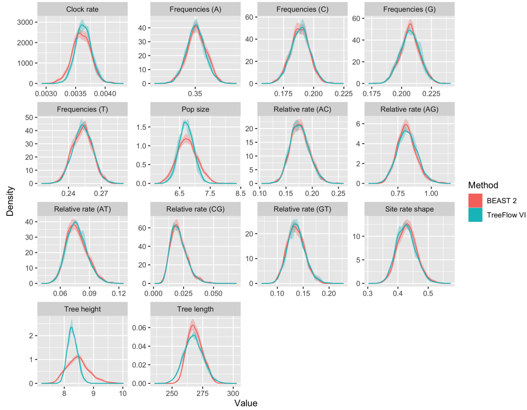
(a) Parameter-marginal Marginal posterior distributions for the model parameters, comparing TreeFlow variational inference (TreeFlow VI, teal) with BEAST 2 MCMC (BEAST 2, red). Shaded bands are Monte Carlo error, obtained as in Figure 2 by bootstrapping for BEAST 2 and from four independent variational runs for TreeFlow VI, whose pooled posterior is the plotted curve. The variational runs use the root full rank approximation; Supplementary Appendix Figure S4 gives the corresponding comparison of all three approximation families.
