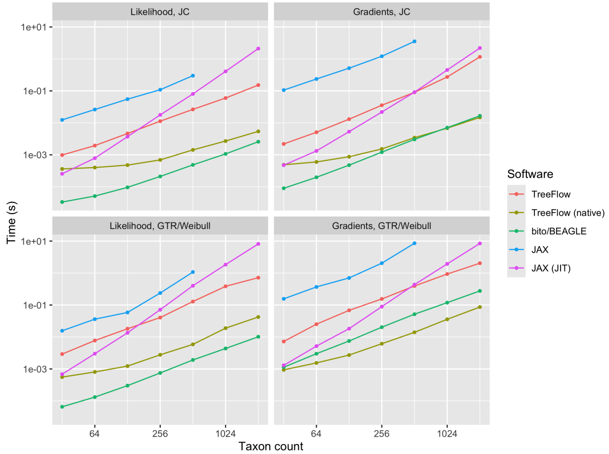
Fig. 5: Times from the phylogenetic likelihood benchmark (100 evaluations, on log-log axes. Each point is the time for a single evaluation of the computation on an alignment of 1000 sites, averaged over 10 simulated datasets. Each panel corresponds to one of the four benchmarked computations (likelihood and gradient evaluation, under the simple JC model and the more complex GTR/Weibull model), with the five implementations plotted as separate series: TreeFlow's portable TensorArray traversal (TreeFlow) and its native C++ operation (TreeFlow (native)), bito/BEAGLE, and the eager (JAX) and JIT-compiled (JAX (JIT)) JAX implementations. Eager JAX is only run up to 512 taxa as its runtime becomes prohibitive on larger trees.
