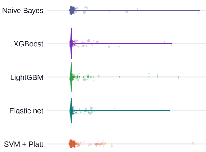
Log loss
