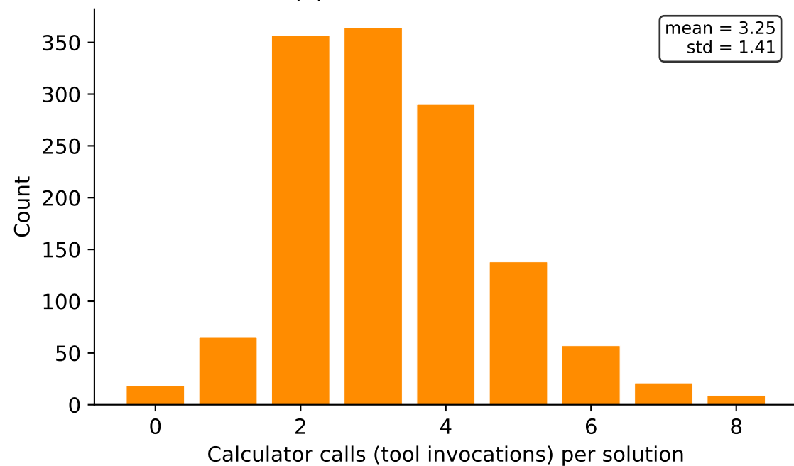
(c) Tool invocation count
