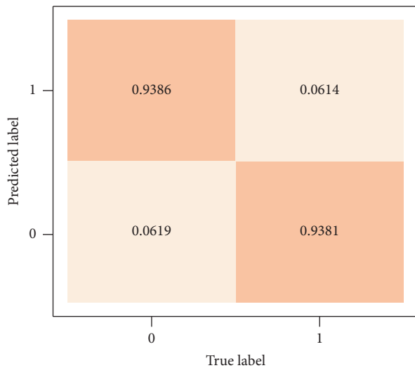
FIGURE 5: Confusion matrix of the proposed approach for classification on INbreast database.
