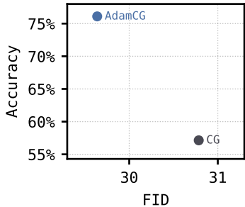
ImageNet Time-Aware Classifier
