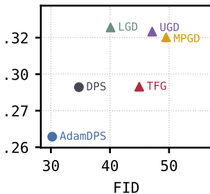
Cats Gaussian Deblur 12
