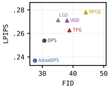
Cats Super Resolution 16x
