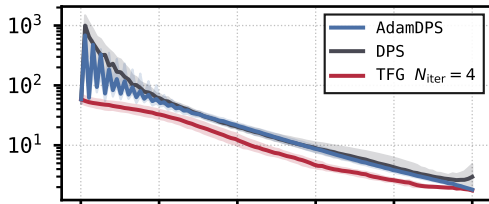
Super Resolution (16x)
