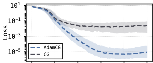
Class-Conditional (Standard Classifier)
