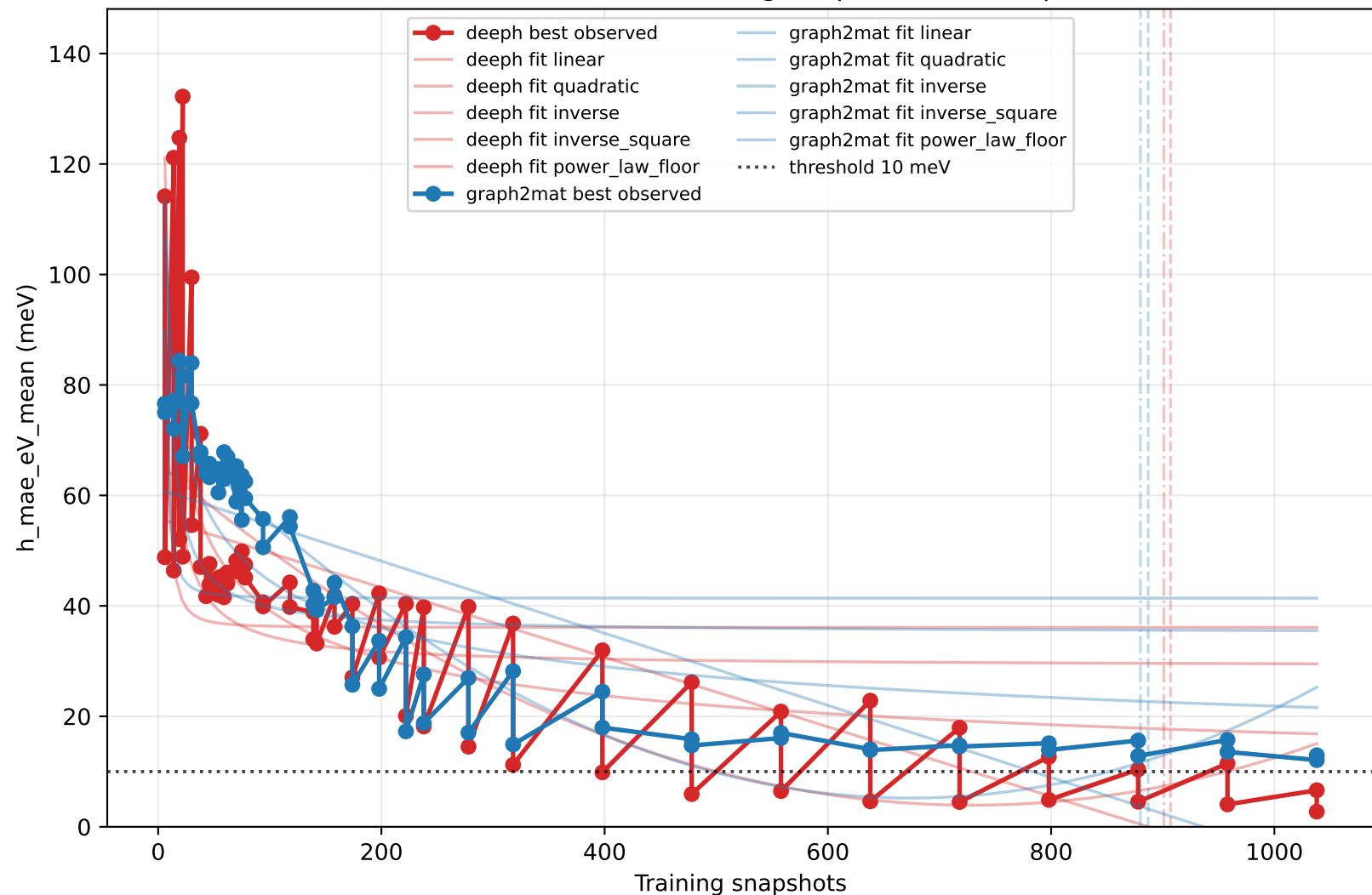
Minimum dataset size from existing Graph2Mat-vs-DeepH metrics
