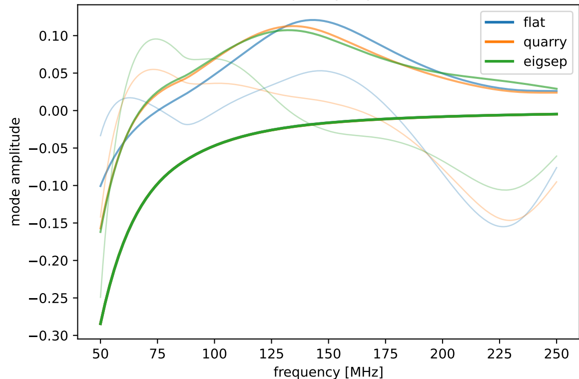
First 3 frequency eigenmodes
