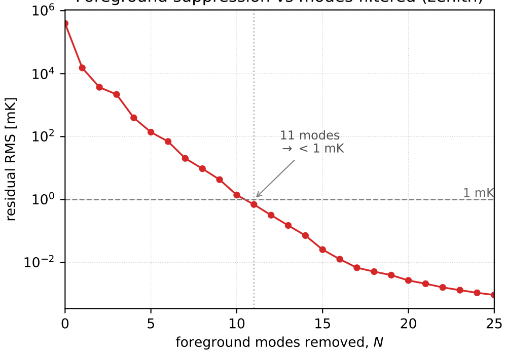
Foreground suppression vs modes filtered (zenith)
