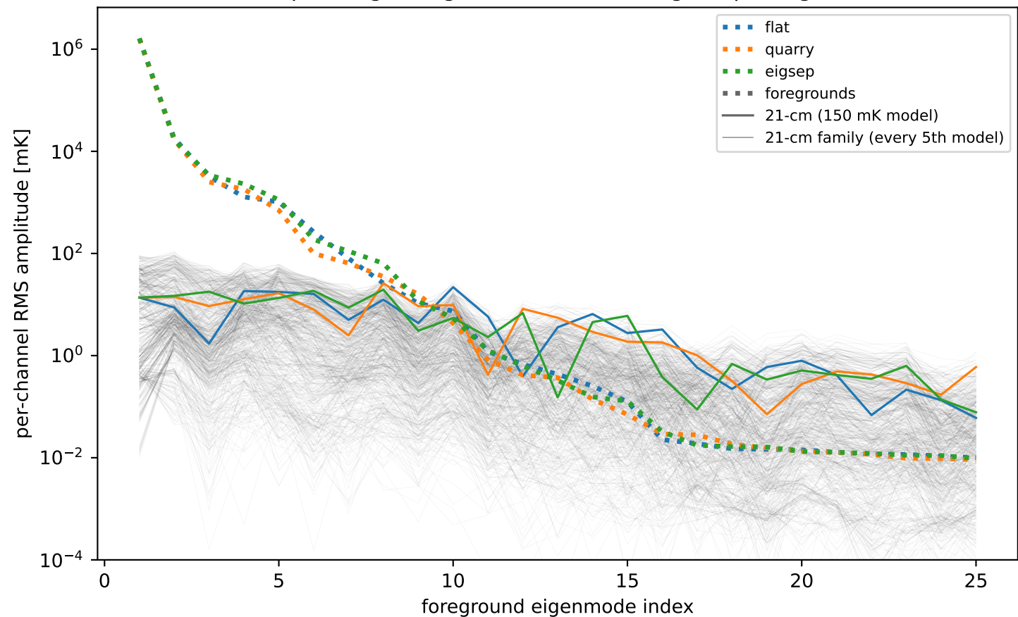
Zenith pointing: foregrounds vs 21-cm signal, per eigenmode
