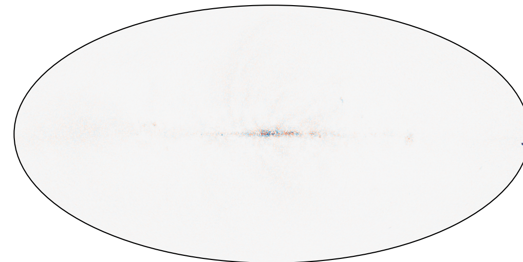
Rotated Stokes U
