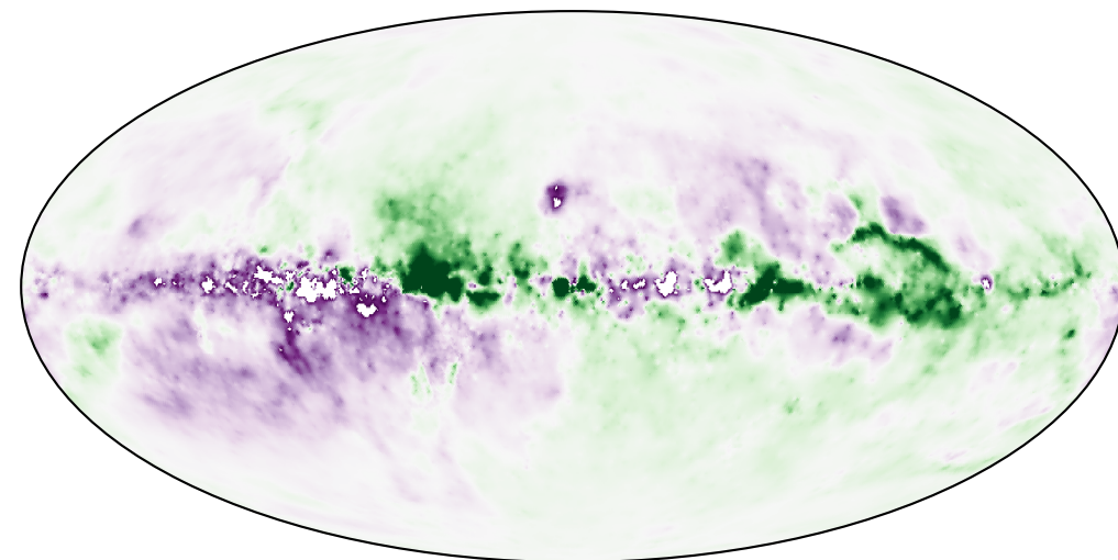
Rotation Measure
