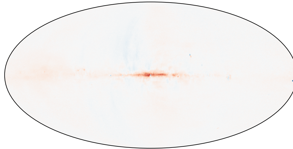
Intrinsic Stokes Q
