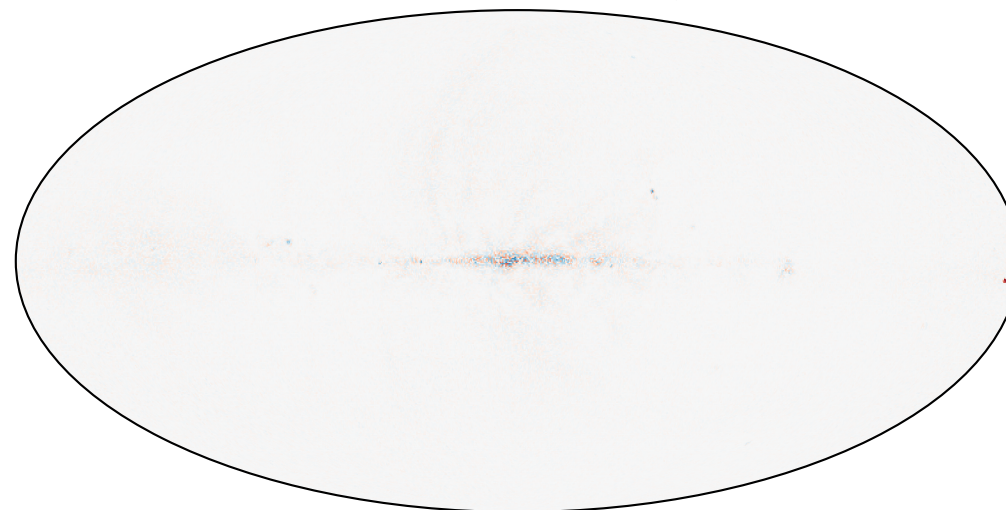
Rotated Stokes Q
