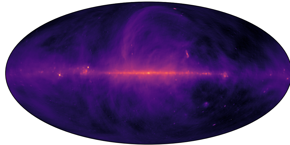
Intrinsic Stokes I (30 MHz)
