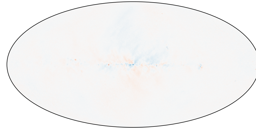
Intrinsic Stokes U
