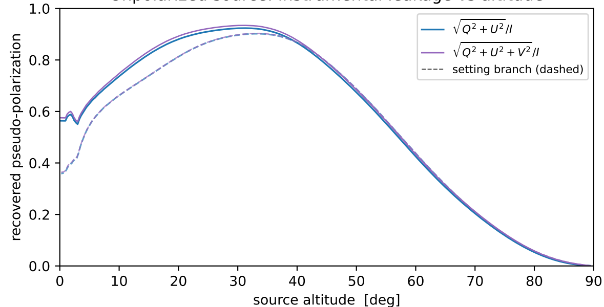
Unpolarized source: instrumental leakage vs altitude
