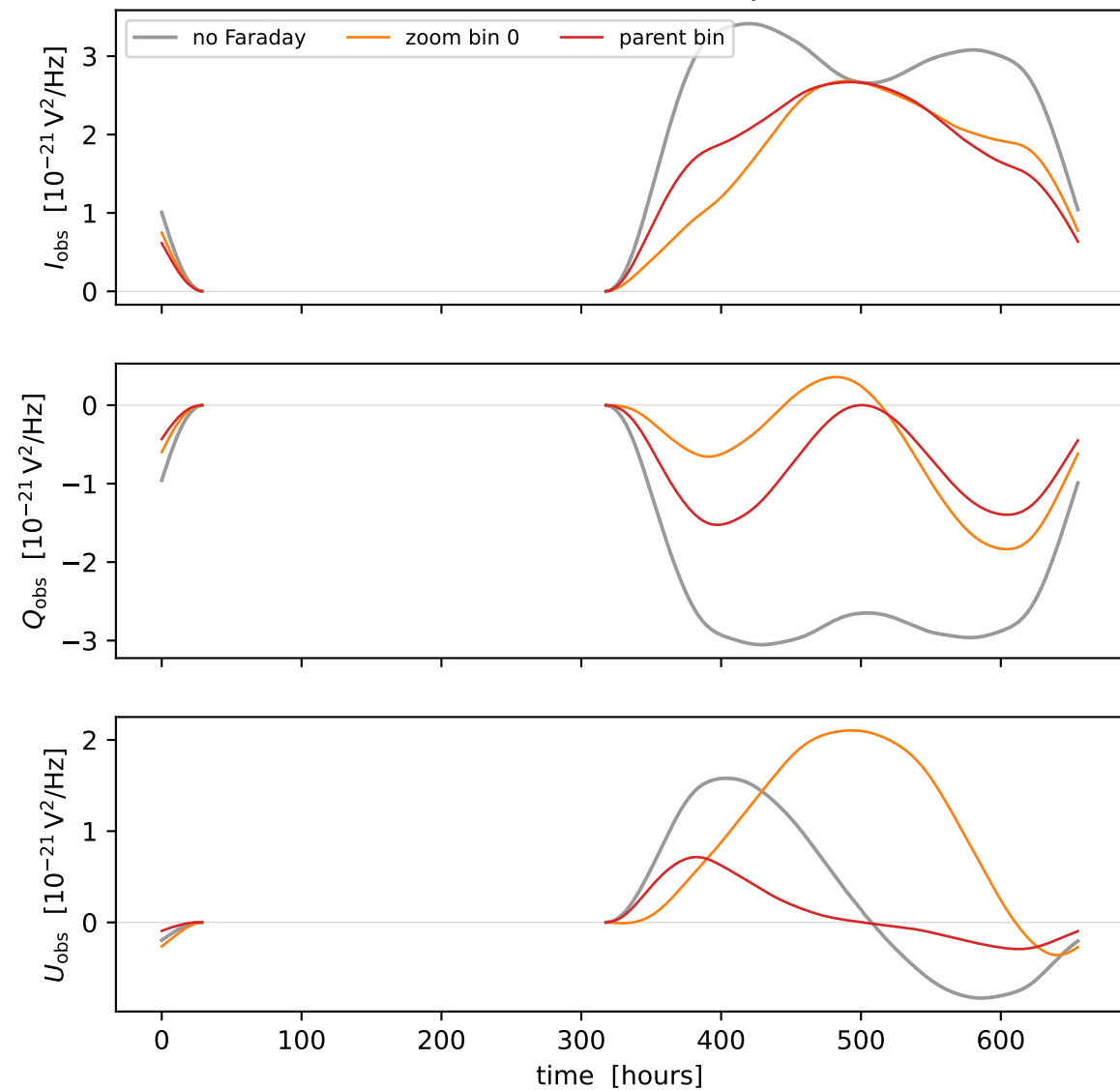
Polarized source track at 30 MHz ( \phi_{\text{FD}} = 250 \text{ rad/m}^2 )
