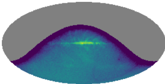
|w|^2 , LST 218 h
