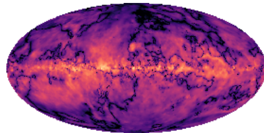
|RM| [rad m -2 ]
