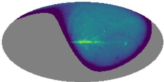
|w|^2 , LST 0 h
