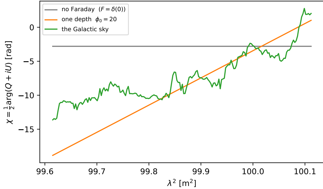
(a) noise-free: Faraday rotation winds \chi linearly in \lambda^2
