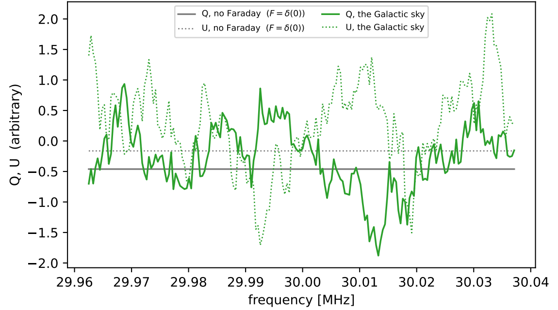
(b) noise-free Q(\nu) , U(\nu) : flat vs decorrelating
