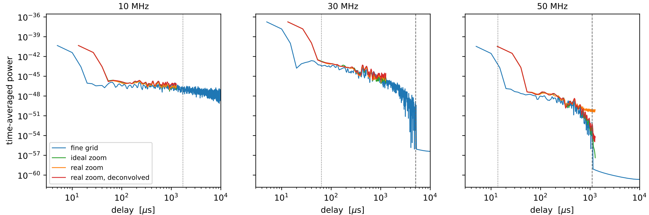
Delay profiles; vertical: \tau_{\text{FD}} for \phi = 30 (dotted) and 2400 \text{ rad/m}^2 (dashed)
