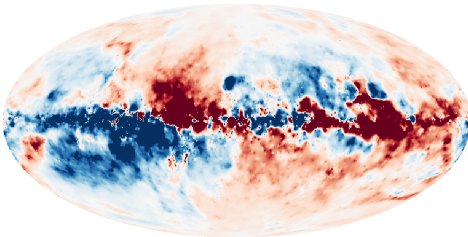
RM [rad/m 2 ]
