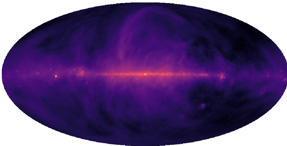
\log_{10} I at 30 MHz [K]
