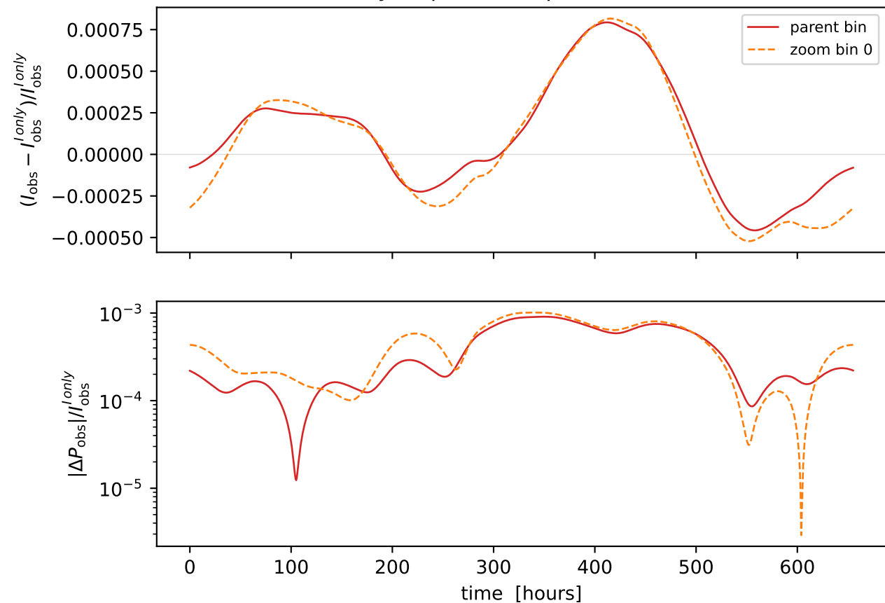
Polarized sky vs perfect depolarization at 50 MHz
