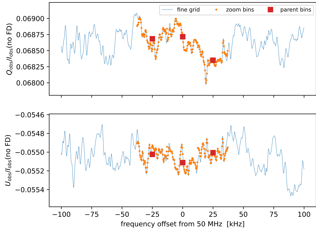
Diffuse sky at 50 MHz, t index 241
