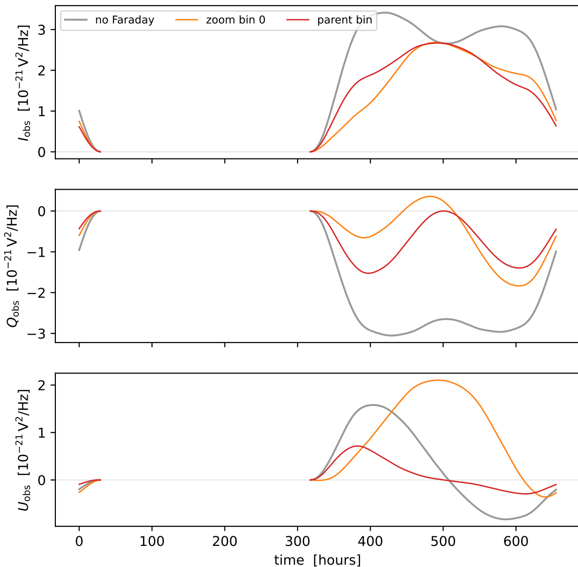
Polarized source track at 30 MHz ( \phi_{\text{FD}} = 250 \text{ rad/m}^2 )
