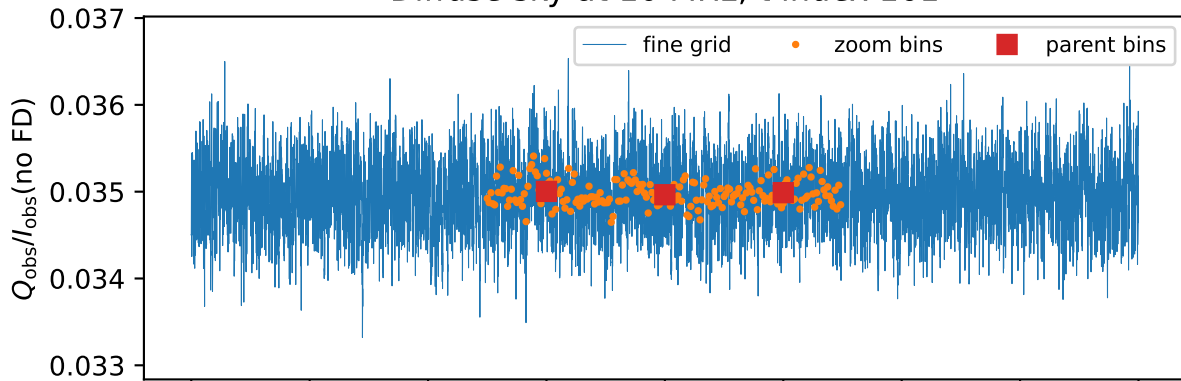
Diffuse sky at 10 MHz, t index 161
